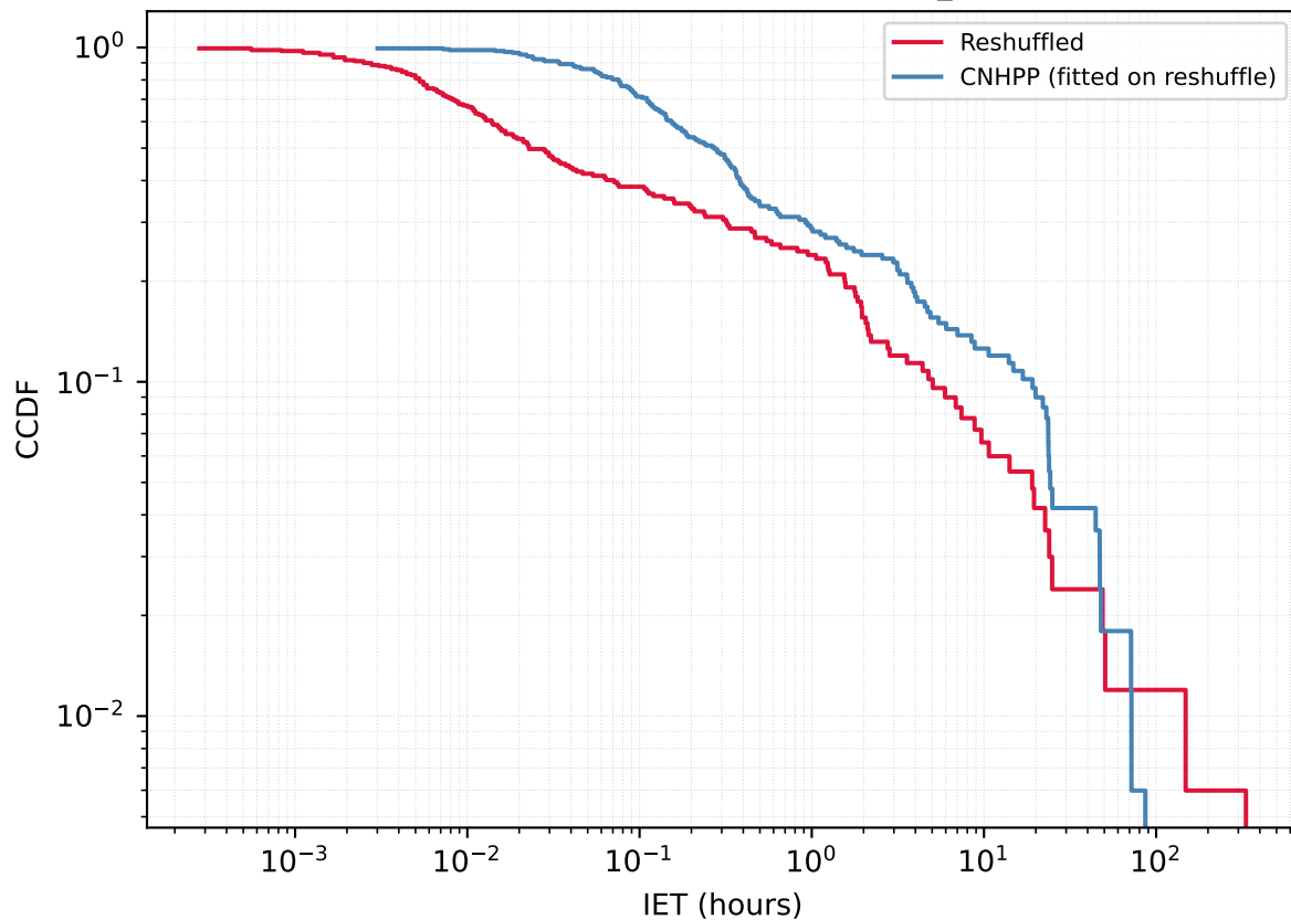
User 57072401 - Reshuffled vs CNHPP A_{\text{fit}}=1.6801
